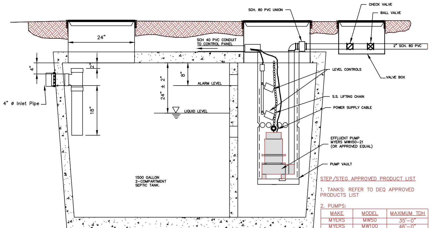
SEPTIC TANK EFFLUENT PUMP INSTALLATION
